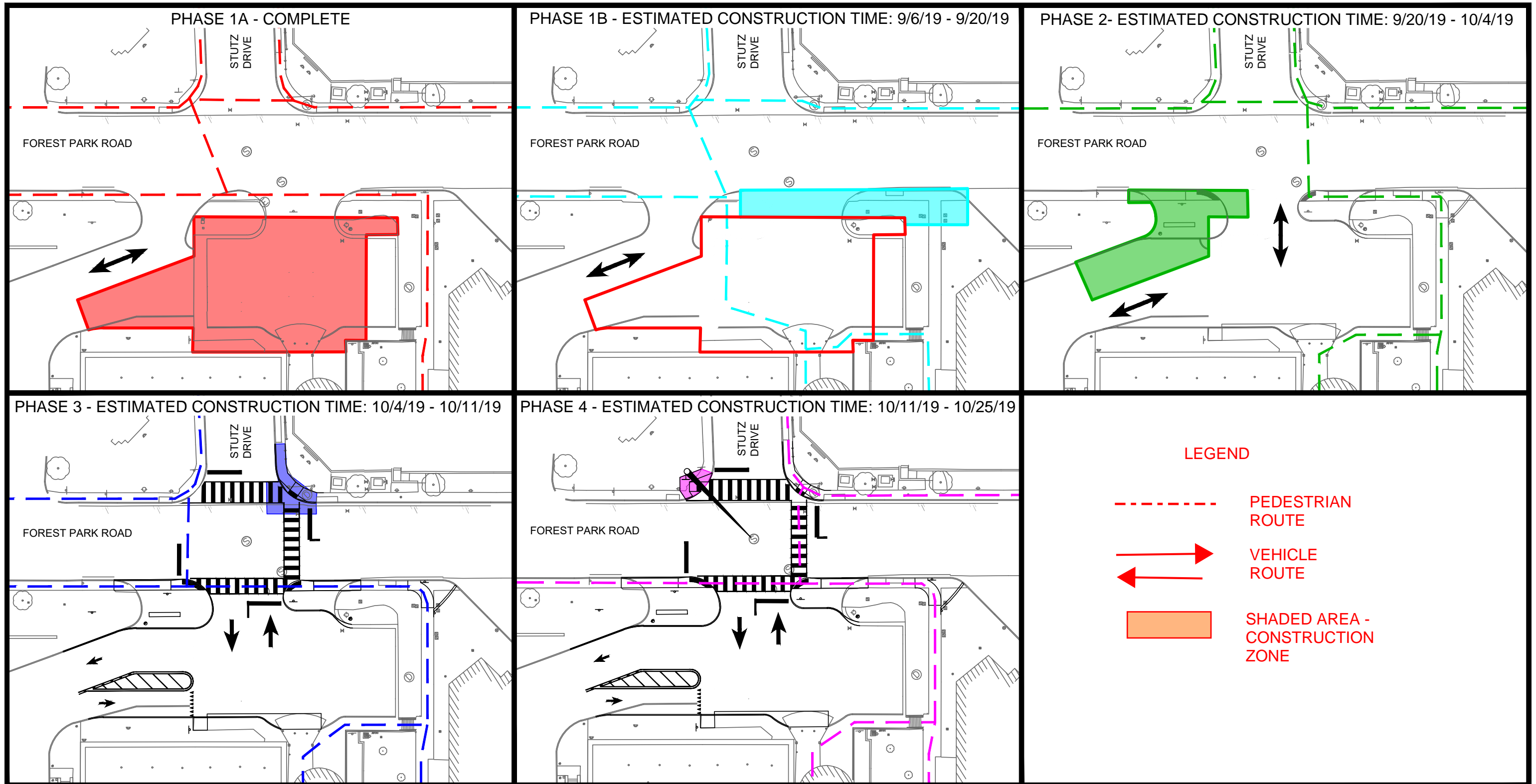
FOREST PARK AND STUTZ DRIVE PHASING PLAN AND PEDESTRIAN ROUTING 9/16/2019
